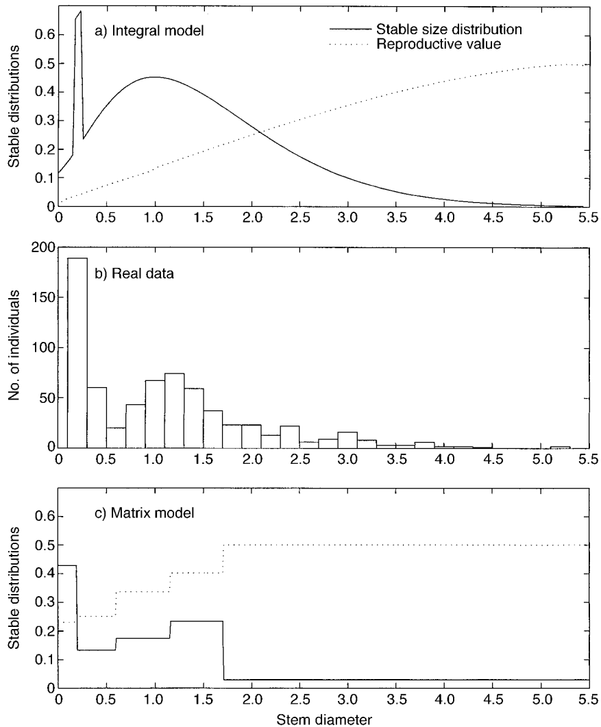
FIG. 4. (a) The stable size distribution (—) and relative reproductive value ( \cdots ) for the integral projection model fitted to the monkshood data. (b) The distribution of plant sizes (stem diameter in millimeters) in the monkshood data set used for fitting the integral projection model. (c) The stable size distribution (—) and relative reproductive value ( \cdots ) for the matrix model given in Eq. 4.
